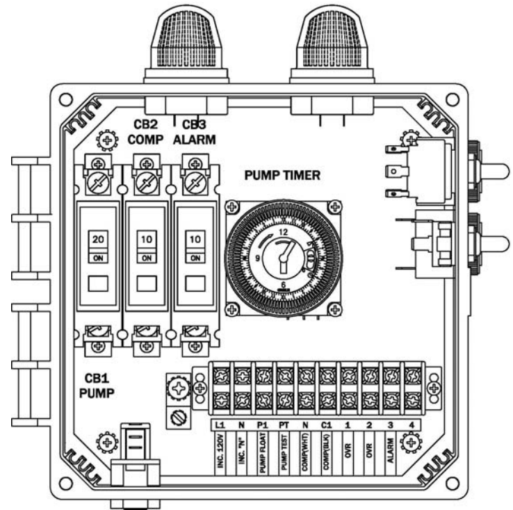
(50B138-A-AV-PT SHOWN)
