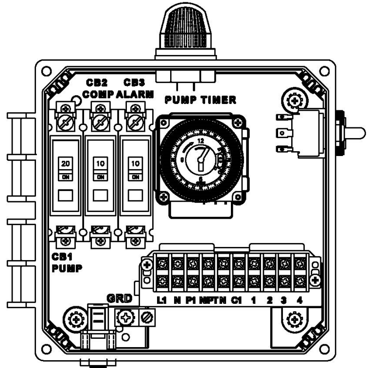
(50B109-CAV SHOWN)
