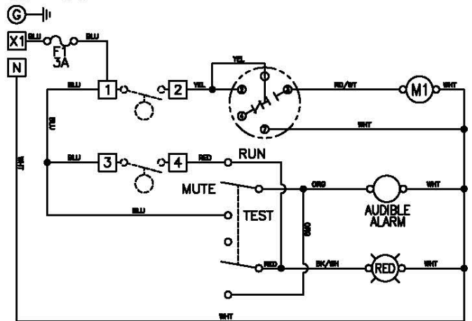
CONTROL POWER CIRCUIT 115 - 1PH
