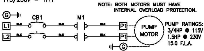
PUMP POWER CIRCUIT 115/230V - 1PH
